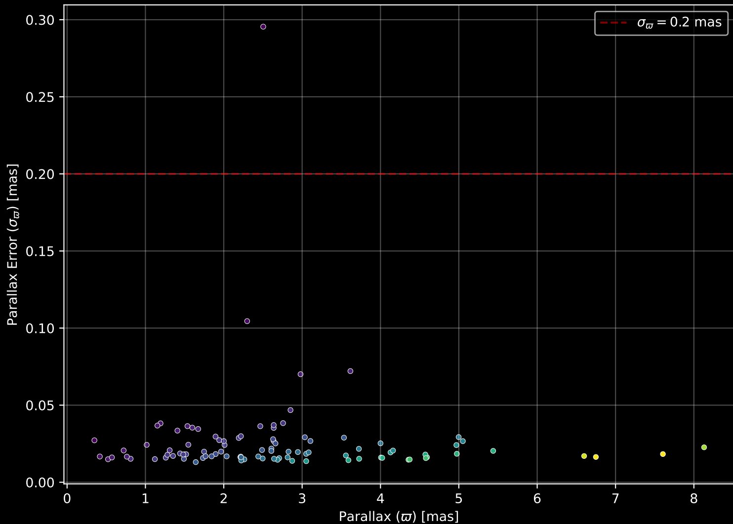
GALAH DR4 Field: [6684] Parallax Quality (n= 97)
