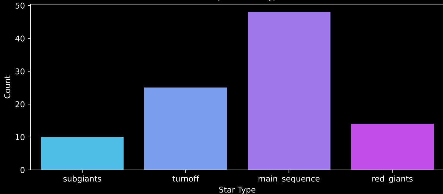
GALAH DR4 Field: [6684] Count plot of Star Type
