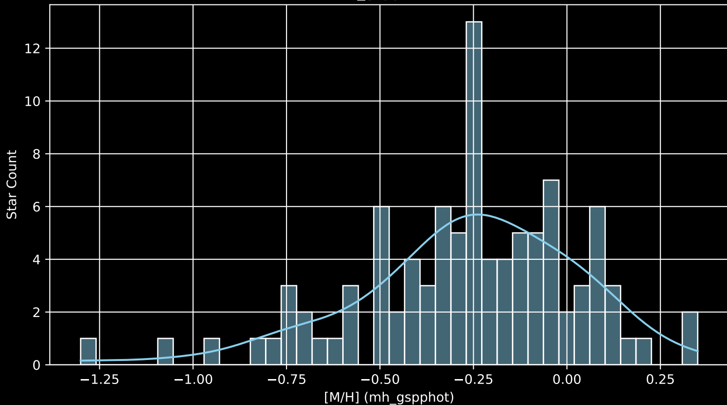
GALAH DR4 Field: [6684] [M/H] (mh_gspphot) (n= 97)
