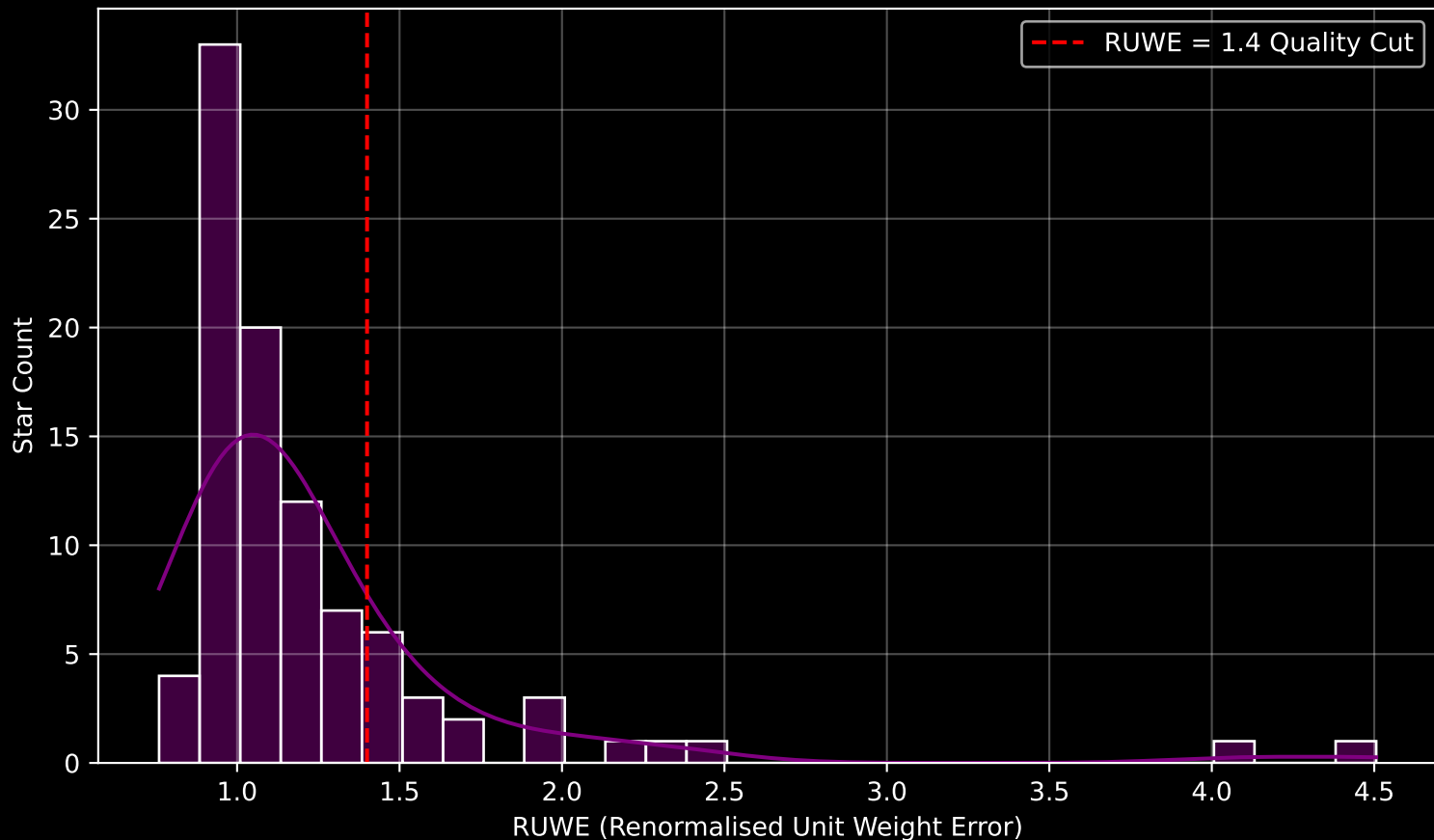
GALAH DR4 Field [6684] RUWE Distribution (n= 95)
