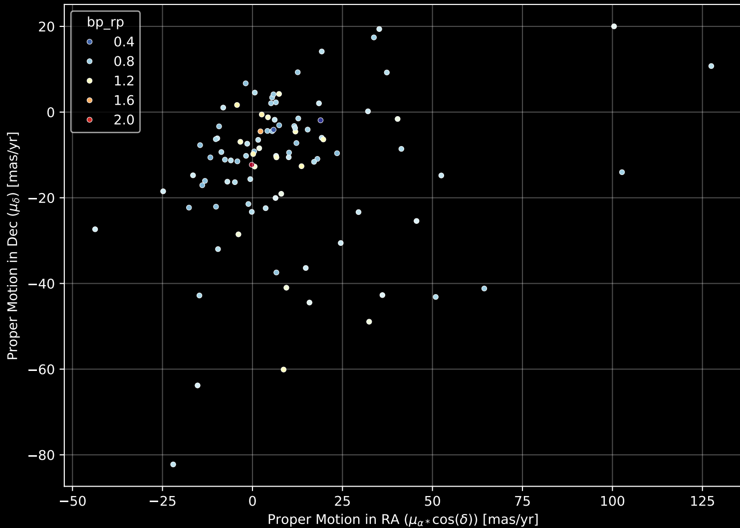
GALAH DR4 Field: [6684] Proper Motion Diagram (n= 97)
